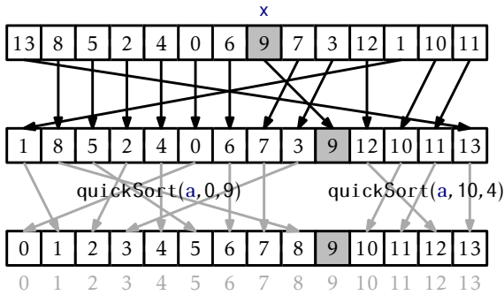
Figure 11.3: An example execution of \text{quickSort}(a, 0, 14)
